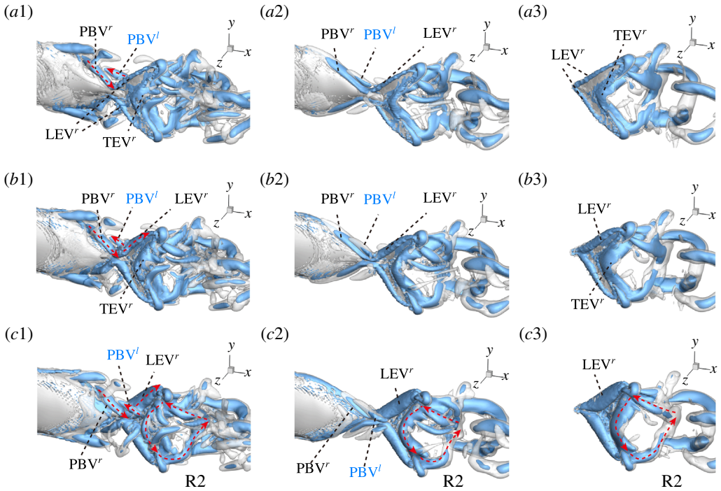
FIGURE 11. (Colour online) Three-dimensional wake structures in M1 ( a1,b1,c1 ), M2 ( a2,b2,c2 ) and M3 ( a3,b3,c3 ) at ( a ) t/T = 0.58 ; ( b ) t/T = 0.67 ; ( c ) t/T = 0.79 . The wake structures are visualized by the isosurface of \lambda_i . |\lambda_i| = 5.6 is for the isosurface in white and |\lambda_i| = 11.2 highlights the vortex core in blue. The arrows indicate the directions of the vortex tubes or vortex rings. CF is flapping rightwards in this figure.
