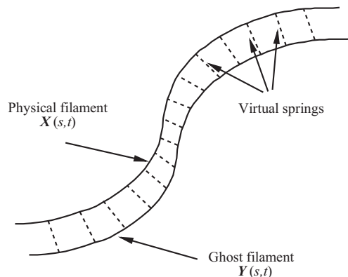
Fig. 2. The physical and ghost filaments are tethered together by virtual springs with a large stiffness K_p .
